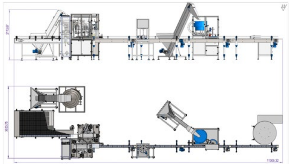
BOV Filling Line up to 40 cans per minute
