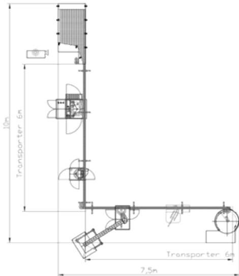
BOV Filling Line up to 25 cans per minute
