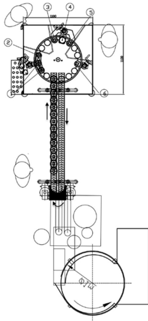
Perfume Filling Line with Buffer Table
